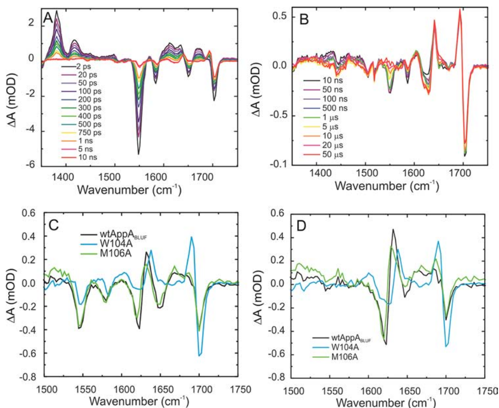
Figure 4. Transient IR spectra for dAppA BLUF and two mutants. (A) Femtosecond to nanosecond TRIR of W104A. (B) Microsecond dynamics of W104A. (C) Comparison of the TRIR spectra of AppA BLUF and the two mutants 10 ns after excitation. (D) As for (C) but 20 \mu\text{s} after excitation.
